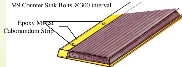
Typical Detail of MODEL "SN-1"
